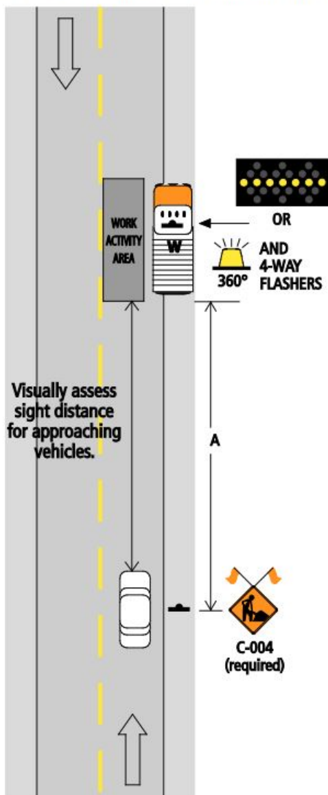
Figure 7.4: Brief-Duration Work – Two-Lane, Two-Way Roadway
